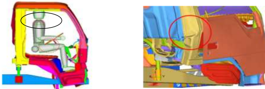
Fig 1 Cabin part intrusion in human dummy due to frontal impact, roof crush and deformation of cabin due to rear impact test
